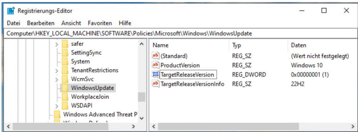
Abbildung 1: Registry Editor (Regedit)
